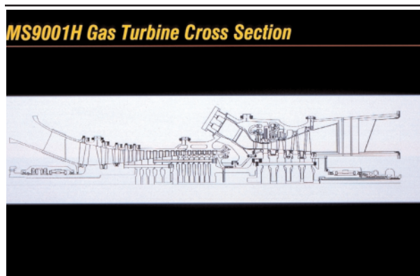
Figure 6. Cross-section H gas turbine
