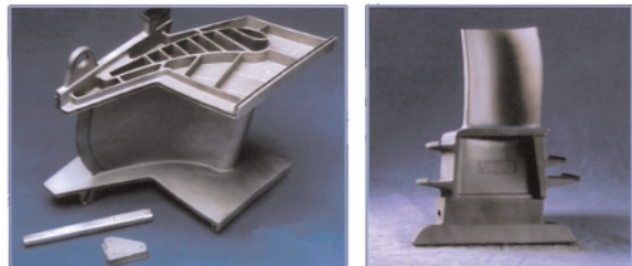
Figure 7. H Stage 1 nozzle and bucket – single crystal
